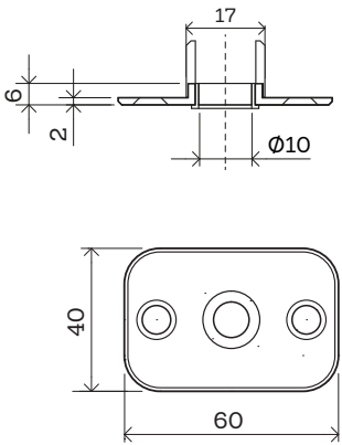
CEILING PLATE
